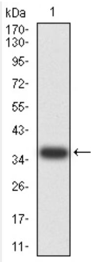
Figure 2: Western blot analysis using PRKAA2 mAb against human PRKAA2 (AA: 453-552) recombinant protein. (Expected MW is 36.7 kDa)
